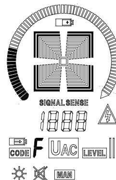
Display FLUKE 2042 Receiver
