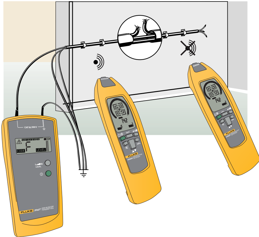
Locating cable interruptions
