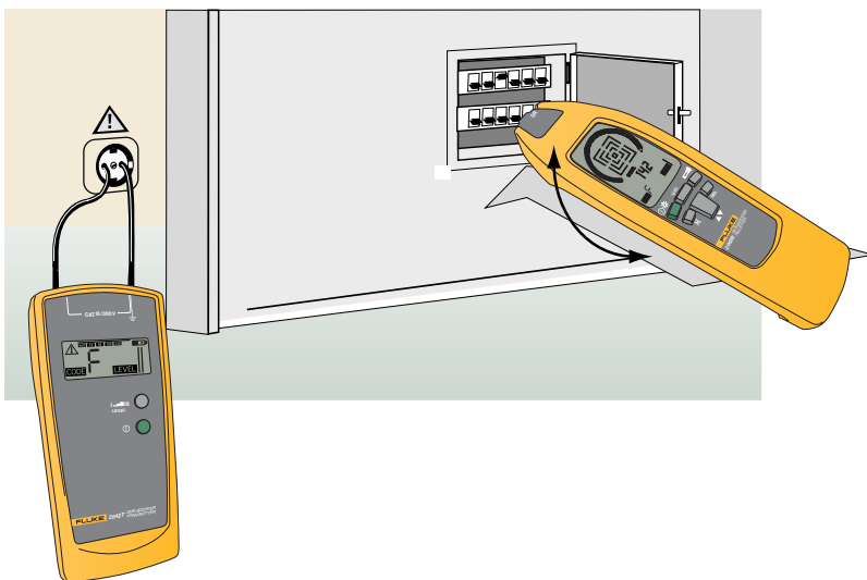
Image 3 - Example of application, allocation from electric circuits to safety devices without switching off the system
