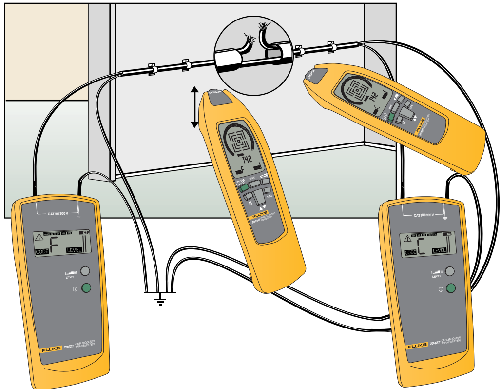
Precise location of interruptions with an additional signal transmitter
