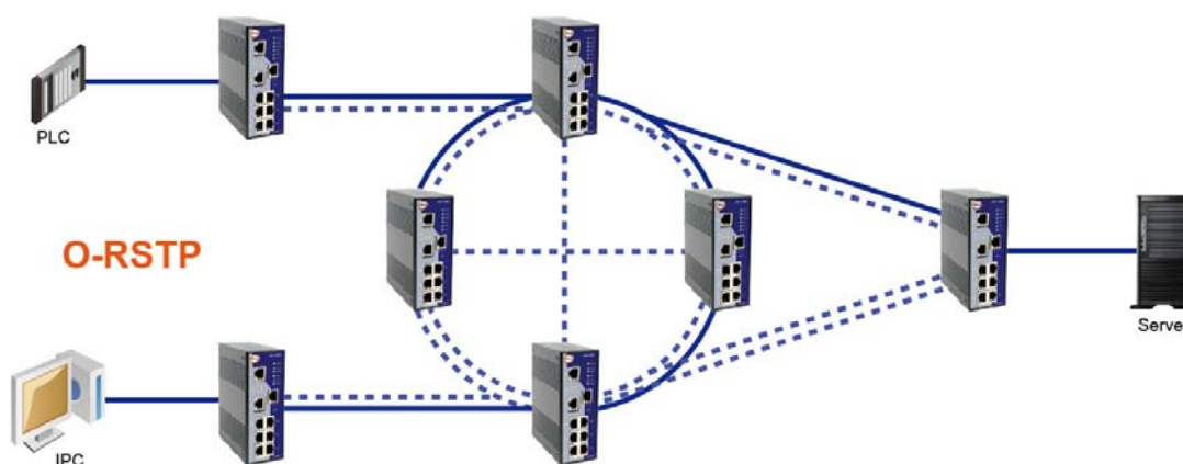
O-RSTP connection
